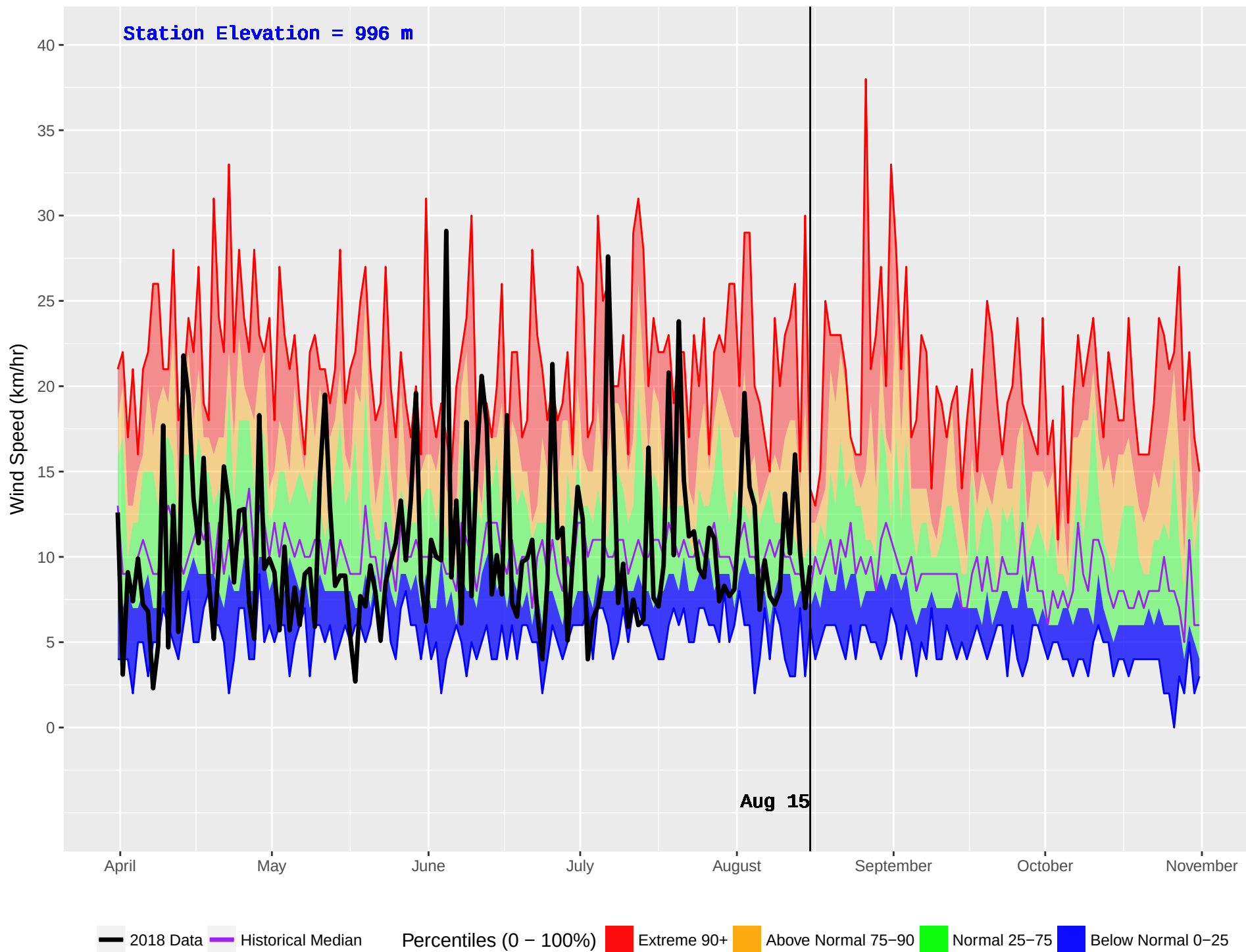
CRANBROOK FS (426) : Historical (2001–2016) and Current (2018) Daily Wind Speed
