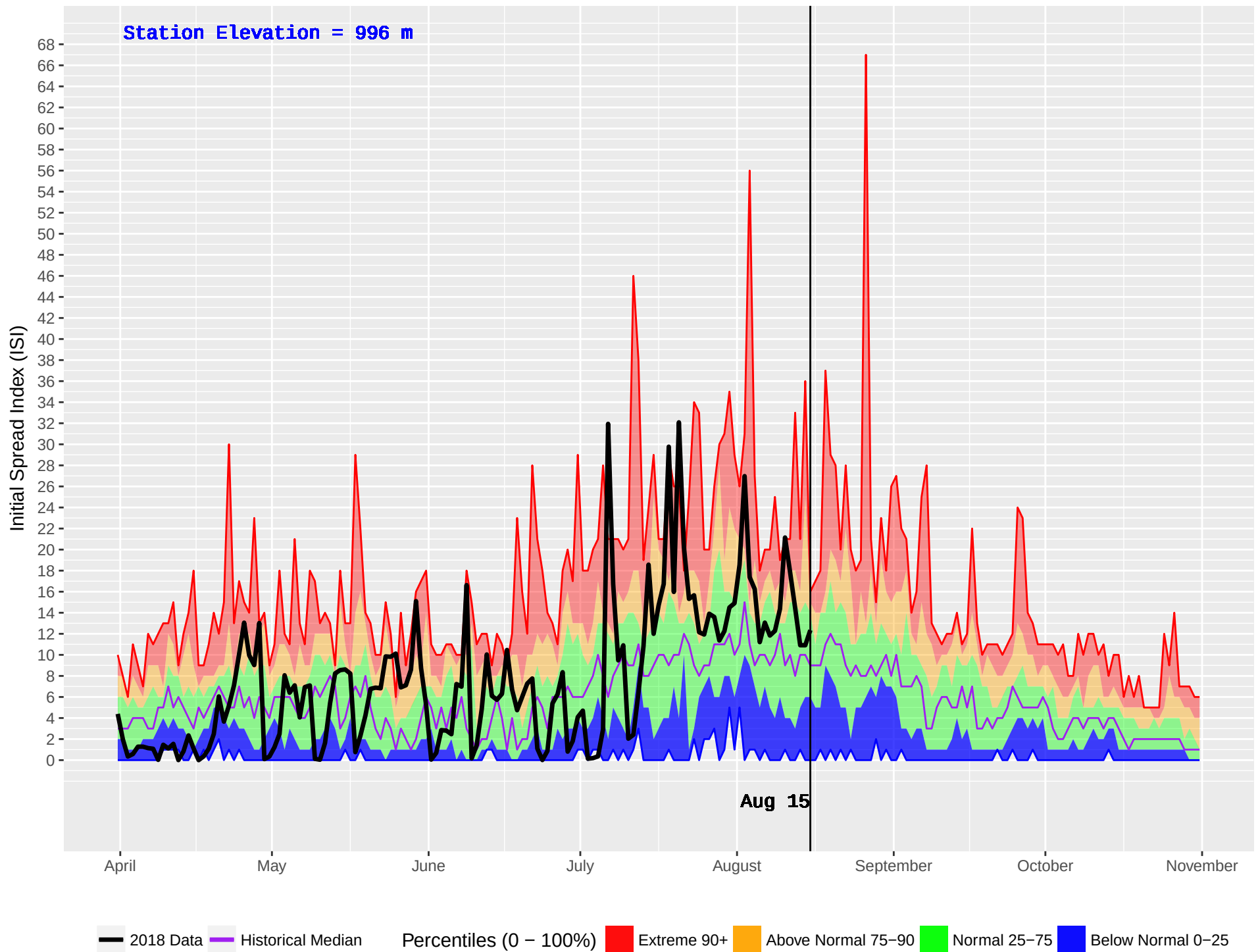
CRANBROOK FS (426) : Historical (2001–2016) and Current (2018) Daily Initial Spread Index (ISI)
