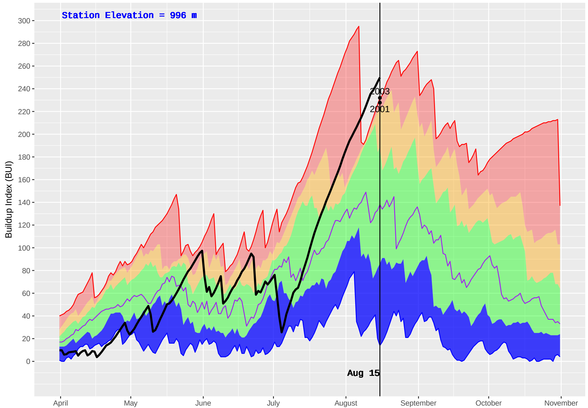
CRANBROOK FS (426) : Historical (2001–2016) and Current (2018) Daily Buildup Index (BUI)
