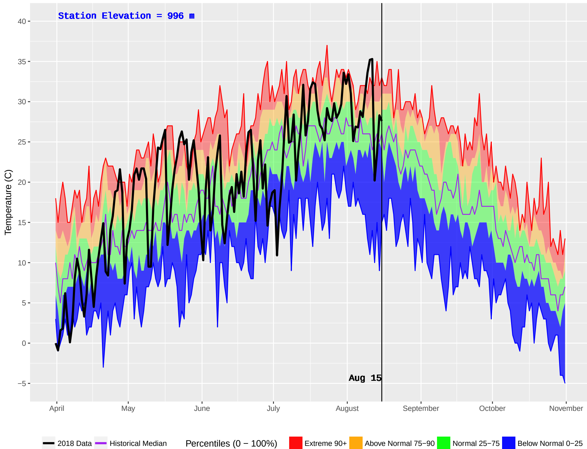
CRANBROOK FS (426) : Historical (2001–2016) and Current (2018) Daily Temperature
